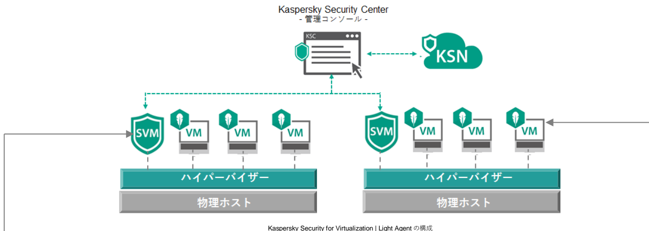
Kaspersky Security for Virtualization | Light Agent の構成
