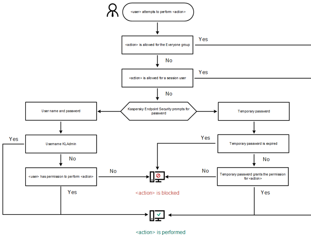
Password protection operating algorithm
