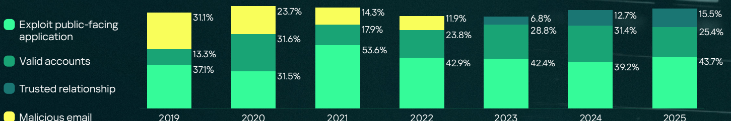
Figure 17 TOP-3 initial attack vectors, 2019-2025
