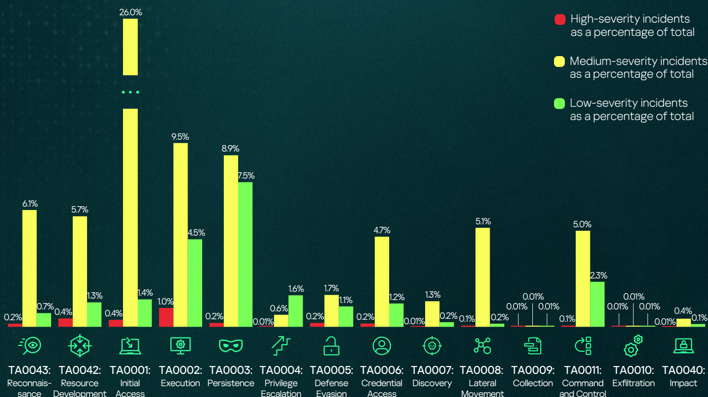
Figure 15 Adversary tactics
